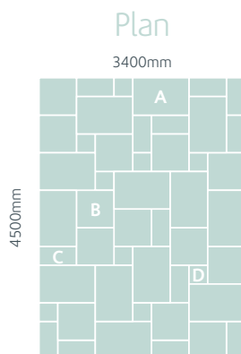
PAVING PAC
